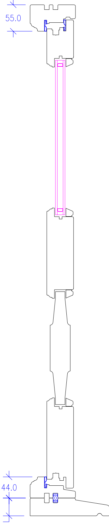
Part Glazed Door With Midrail And 42mm Raised And Fielded Timber Panel. Vertical Section
