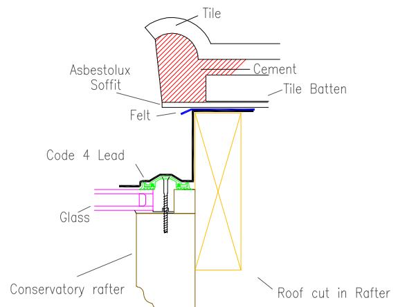
Roof Cut In Rafter Joining Detail
