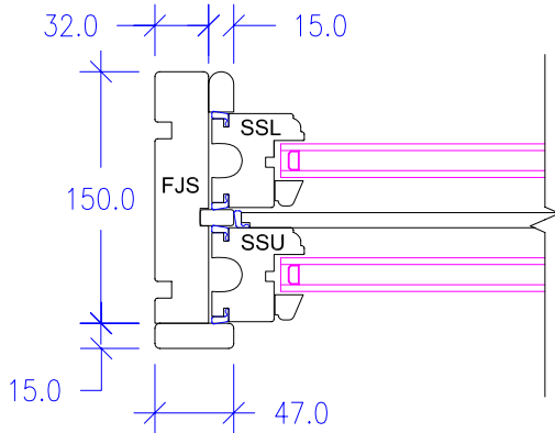
Horizontal Section-Spiral Balances
