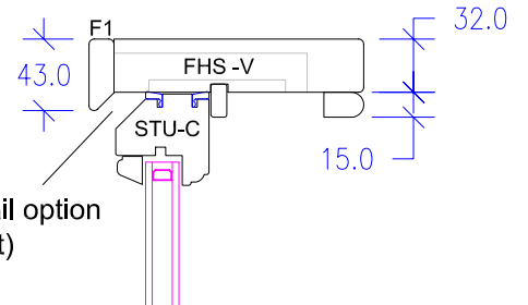
Top Rail with Trickle Vent (Spiral Balanced)
