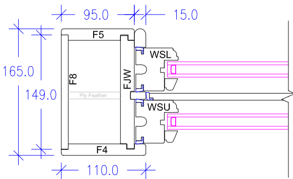
Horizontal Section-Weights & Pulleys
