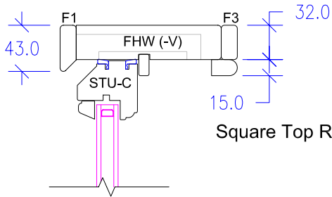
Option to have Top Rail equal to side boxes on Weights and Pulleys version
