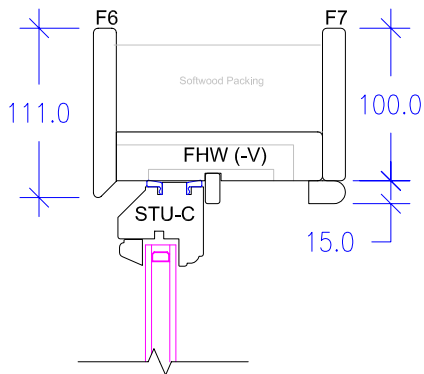
Horizontal Section-Spiral Balances
